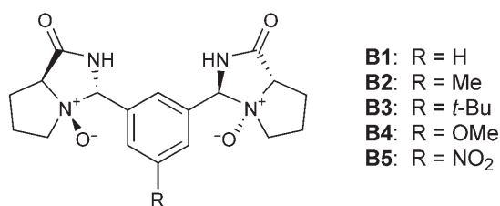
Figure 1. Structures of catalyst series B .
