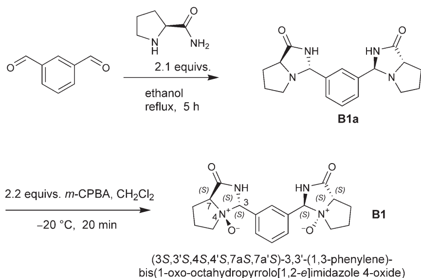
Scheme 2. Preparation of catalyst B1 .
