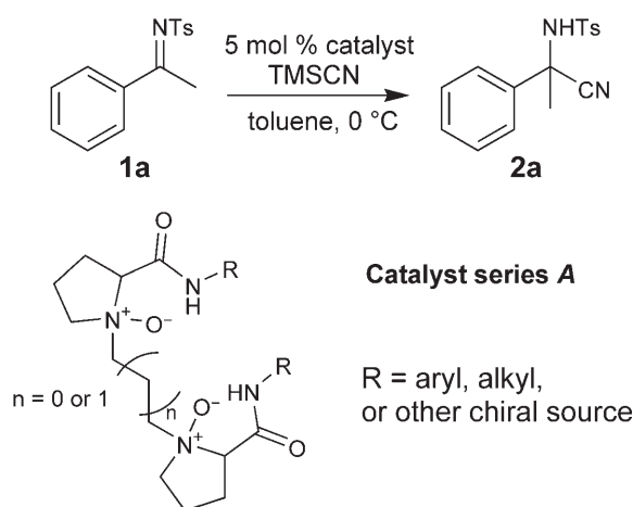
Scheme 1. Catalytic asymmetric cyanation of ketoimine 1a using the catalyst series A .
