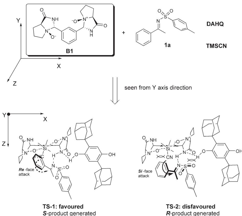
Figure 2. A simplified model of proposed transition state.
